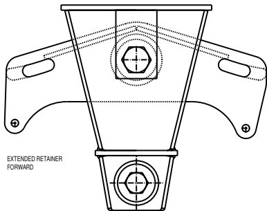
EQUALIZER & BRACKET ASSEMBLY 44" AXLE SPACING
