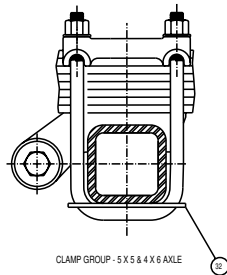
CLAMP GROUP - 5 X 5 & 4 X 6 AXLE
