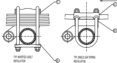
TYP. INVERTED U-BOLT INSTALLATION
